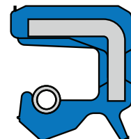
Design BA..SL Conforming to DIN/ISO Design AS Smooth OD
