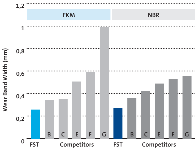
Average wear band of radial shaft seals (Standard test in mineral oil)
