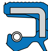
Design BA..SL Conforming to DIN/ISO Design AS Grooved OD
